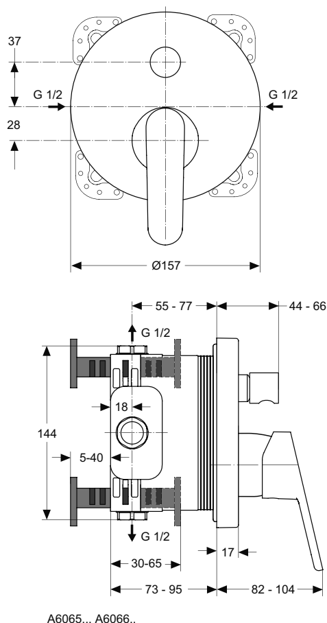
A6065.., A6066..
